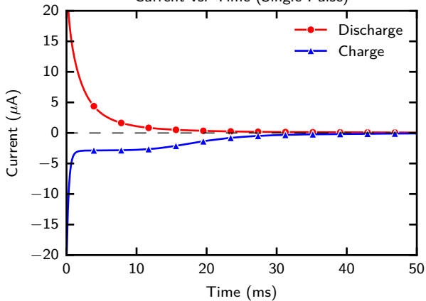
Current vs. Time (Single Pulse)
